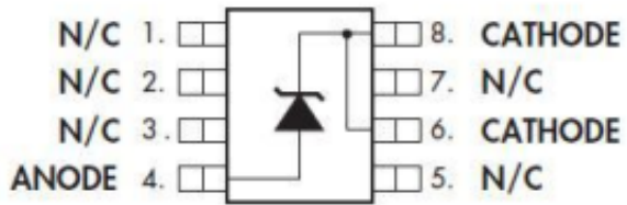
DM PACKAGE (Top View)
